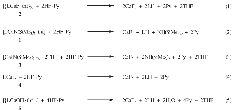
Scheme 2. Reactions of HF·Py (Py = pyridine) with the soluble calcium compounds 1 – 5 .
